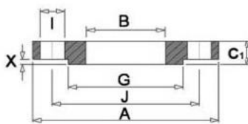
Plate Flange
