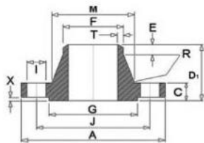
Weld Neck Flange
