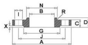
Slip-On Flange
