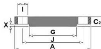
Blind Flange
