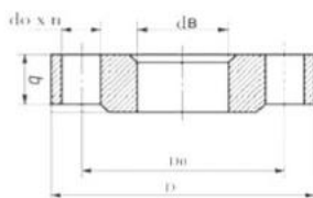
Flat Face Flange
