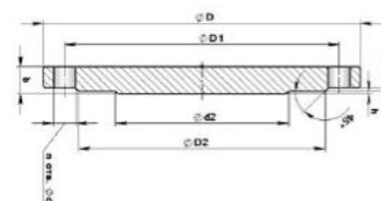
Blind Flange
