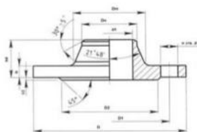
Weld Neck Flange
