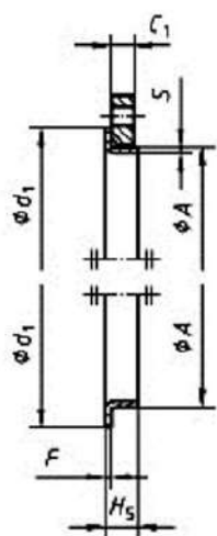
Type 02 and 37
