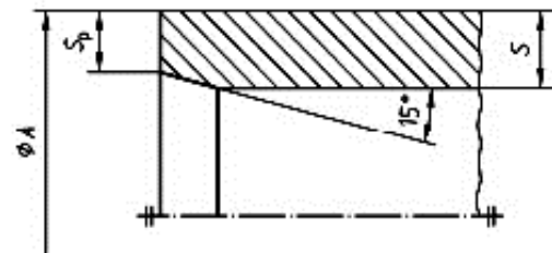
Chamfer B
