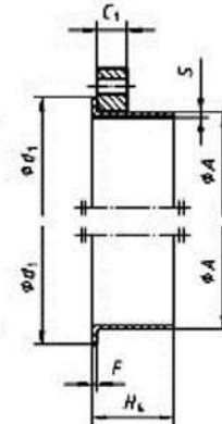
Type 02 and 36
