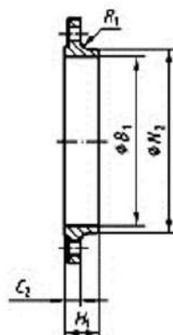
Type 12
