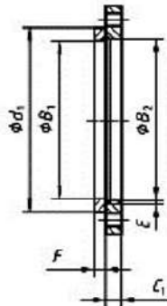
Type 02 and 32
