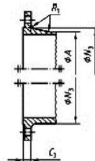
Type 21
